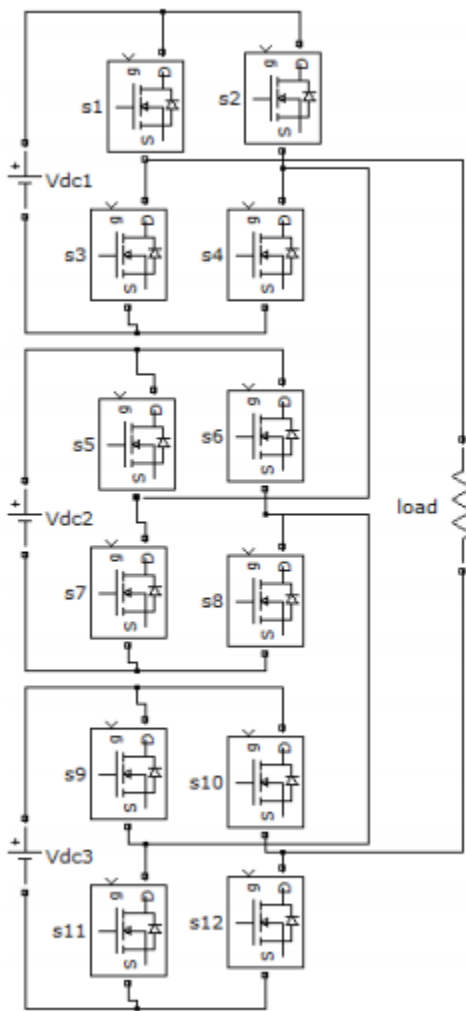
Fig. 1: Single phase 7-level inverter
