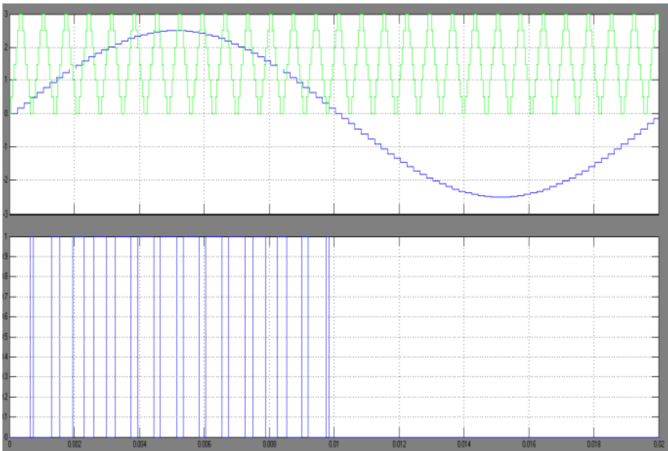
Fig. 3: Simulation output of 2-level positive cycle SPWM
