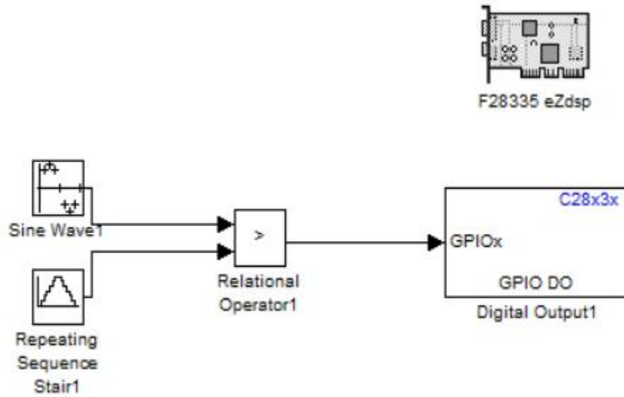
Fig. 2: SIMULINK block diagram to generate SPWM
