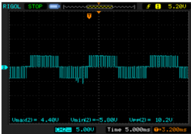
Fig. 5: 2-level inverter hardware output
